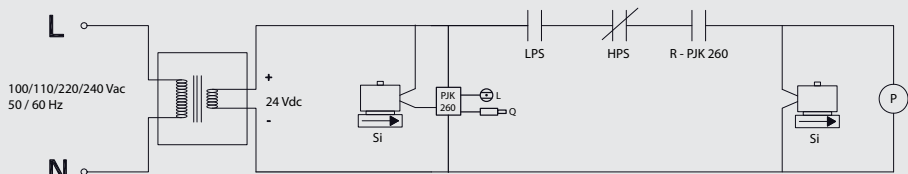
Electrical diagram
