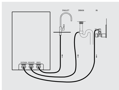
Hydraulic connections diagram
